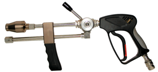
CONfire Nozzle NFF-NZ-CFN
