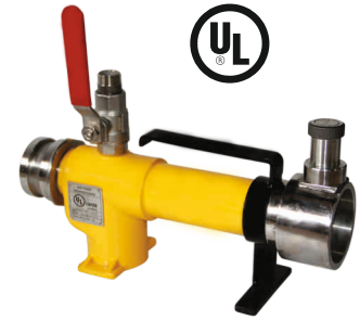
Inline Inductor NewAge-ILI-225-f / 450-F
