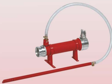
Inline Foam Generator NFF-FE-FGI
