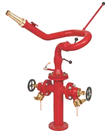
2 - Way Stand Post with Monitor SPH-2WM
