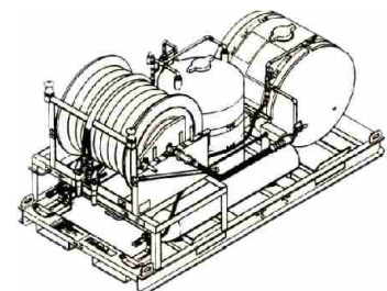
Twin Agent Skid
