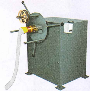
Electrical Hose Binding Machine NFF-HME-EHBM
