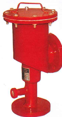
Foam Maker with Vapor Seal Chamber NFF-FE-FMWVS
