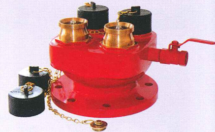
Four Way Inlet Breaching NFF-DRE-4W
