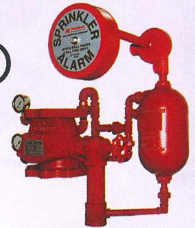
Alarm Valve NewAge-AV-4 / 6
