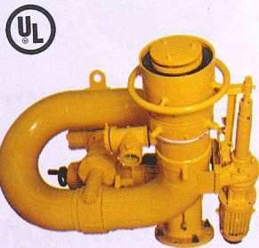
Fixed / Adjustable Flow Monitor UL Listed
