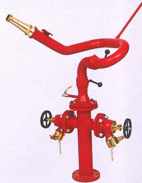
2 - Way Stand Post with Monitor NFF-SPH-2WM
